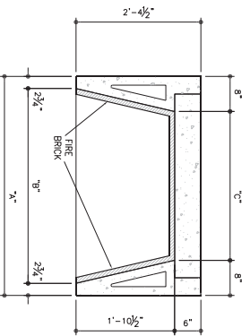
FIREBOX PLAN SCALE: 3/4" = 1'-0"
