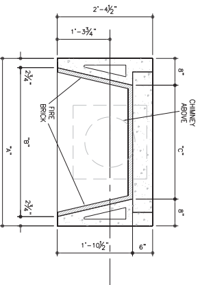
FIREBOX PLAN SCALE: 1" = 1'-0"
